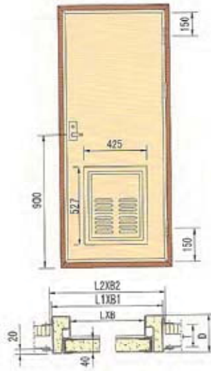
B15-S 带应急逃生风栅 B15-S WITH F-F VENT LOUVER
