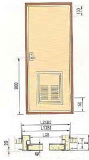
B0-S 带应急逃生风栅 B0-S WITH E-E VENT LOUVER
